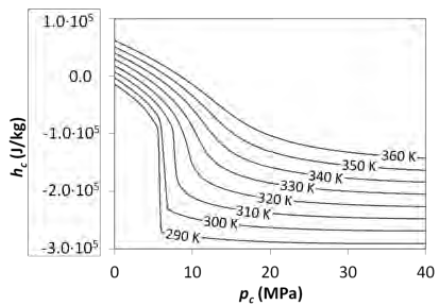
Redlich-Kwong EOS (1949)
