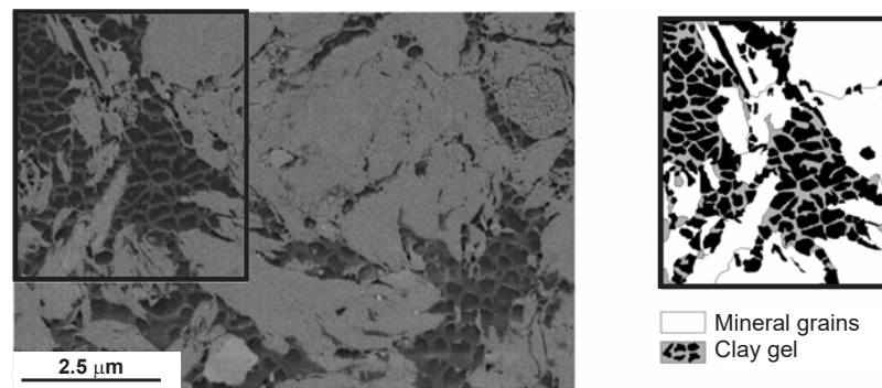
Figure 13: Microstructure of compacted MX-80 bentonite with dry density \rho_d = 1.46 \text{ Mg/m}^3 and water content w = 22.6\% obtained by cryo-Focused Ion Beam nanotomography [Keller et al. , 2014].
