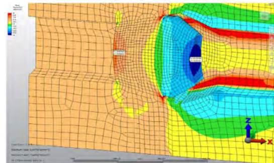
Posiva's Wedge Plug design (top) & water pressure simulations in FEM modeling (bottom)
