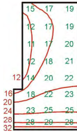
Water content [%]
