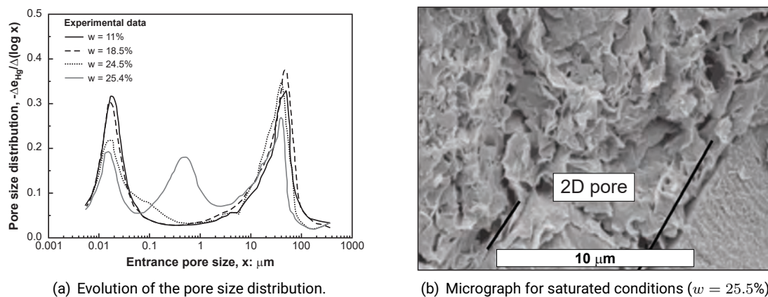
Figure 14: Development of two-dimensional fissure like pores during hydration of a MX-80 bentonite/sand mixture under constant volume conditions [Wang et al. , 2013a]
