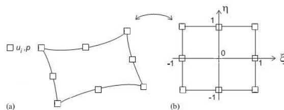
(a) Quadrilateral element
