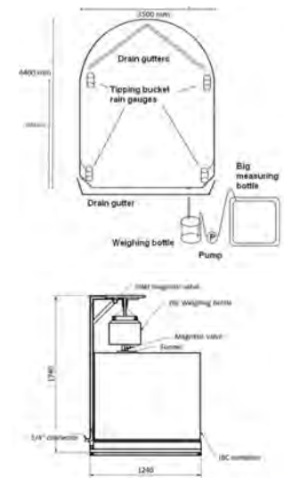
Schematic illustration of the design of the leakage measurement system. (© VTT)
