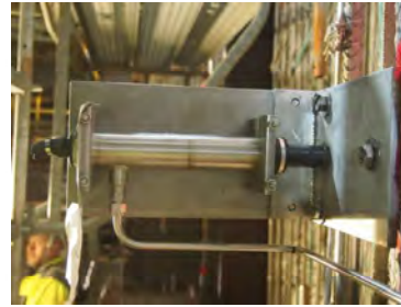
Displacement sensors at the back face of the plug and specially designed sensor holder
