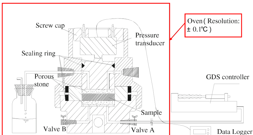
Constant volume swelling cell
