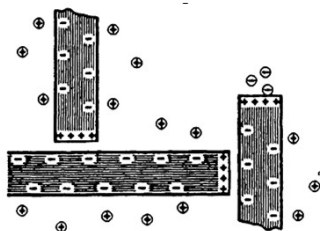
Coulomb attraction
