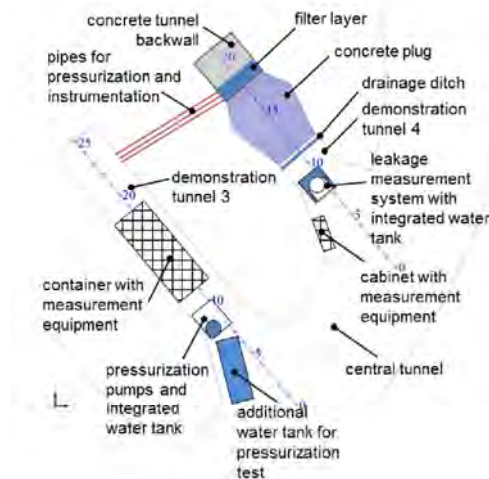
Horizontal section of demo tunnels 3 & 4 with concrete plug and locations of instrumentation equipment
