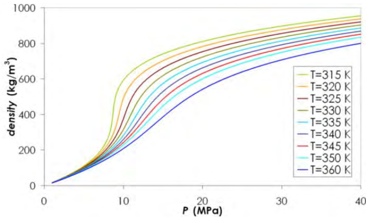
Redlich-Kwong EOS with Spycher et al. (2003) parameters
