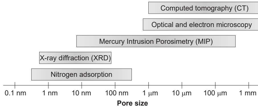
Figure 7: Range of applications of various experimental techniques used to investigate the microstructure of porous materials.
